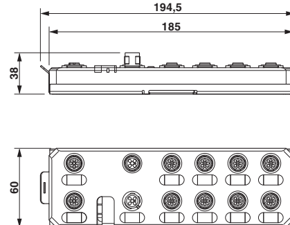
Dimensional drawing
